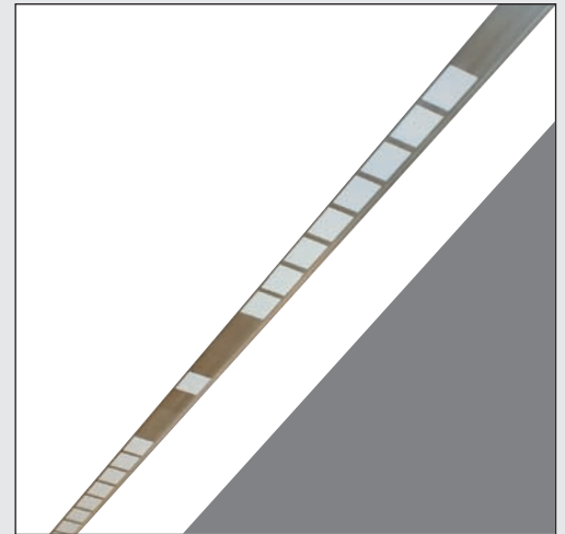
BL 1013 Recessed Beamlight with 2x5312 OP and 1x5306 (2x26W-PL)
